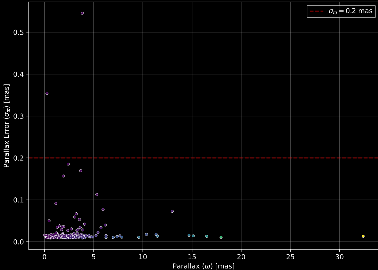
APOGEE DR17 Field: [085+35_MGA] Parallax Quality (n= 193)
