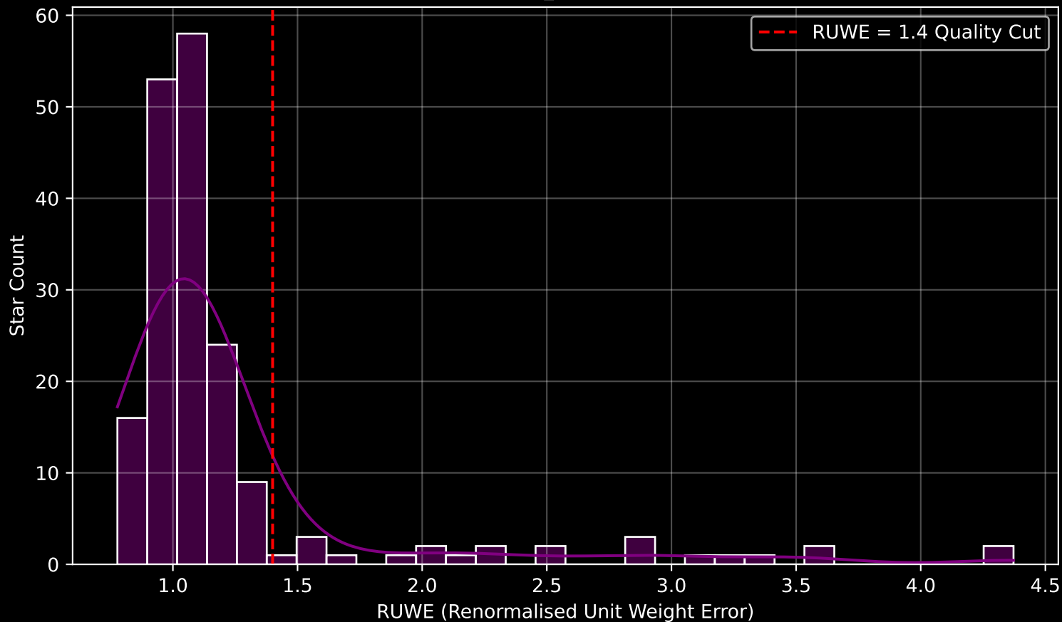
GAPOGEE DR17 Field [085+35_MGA] RUWE Distribution (n= 183)
