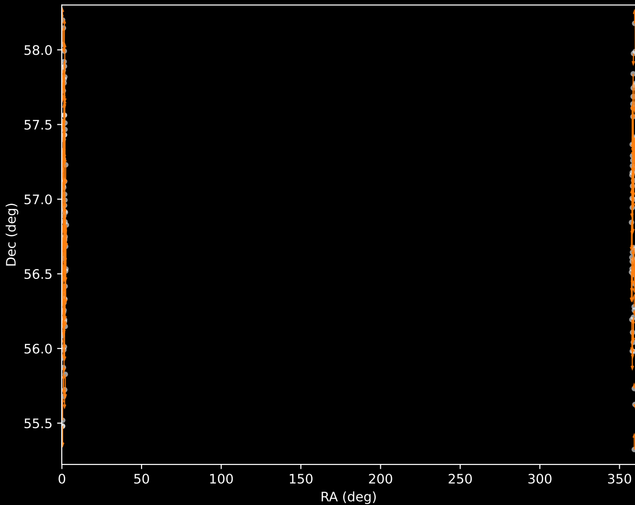
APOGEE DR17 Cluster 2 Proper Motion Vectors (n=126)
