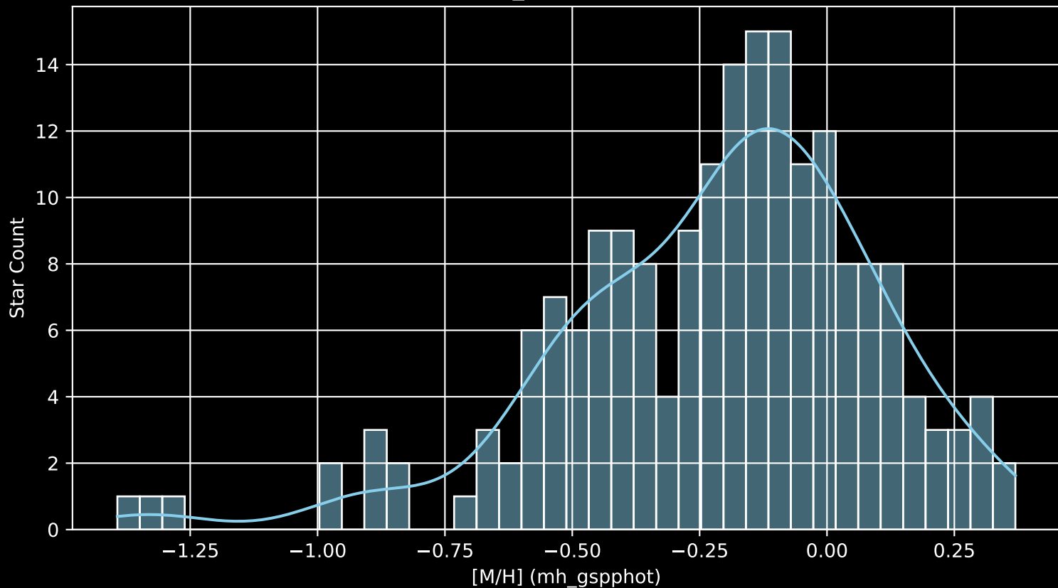
APOGEE DR17 Field: [085+35_MGA [M/H] (mh_gspphot) (n= 192)
