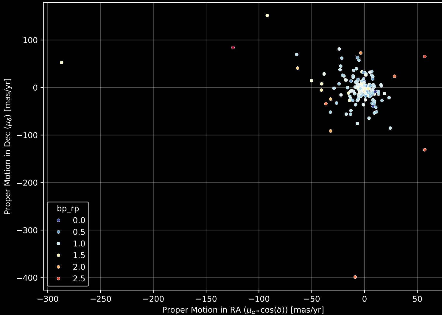
APOGEE DR17 Field: [085+35_MGA] Proper Motion Diagram (n= 193)
