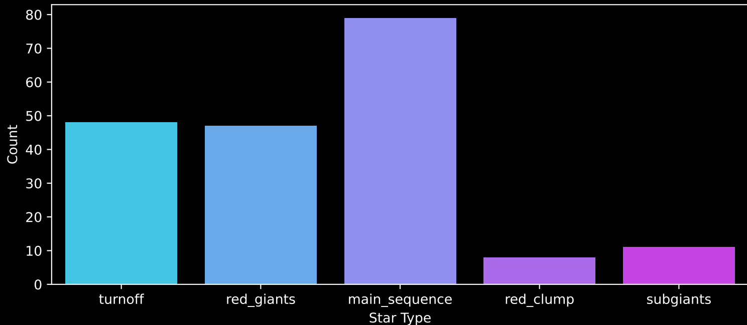
APOGEE DR17 Field: [085+35_MGA] Count plot of Star Type
